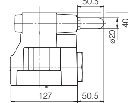
AGIS-20; Mass = 6 Kg AGIU-20; Mass = 6 Kg
